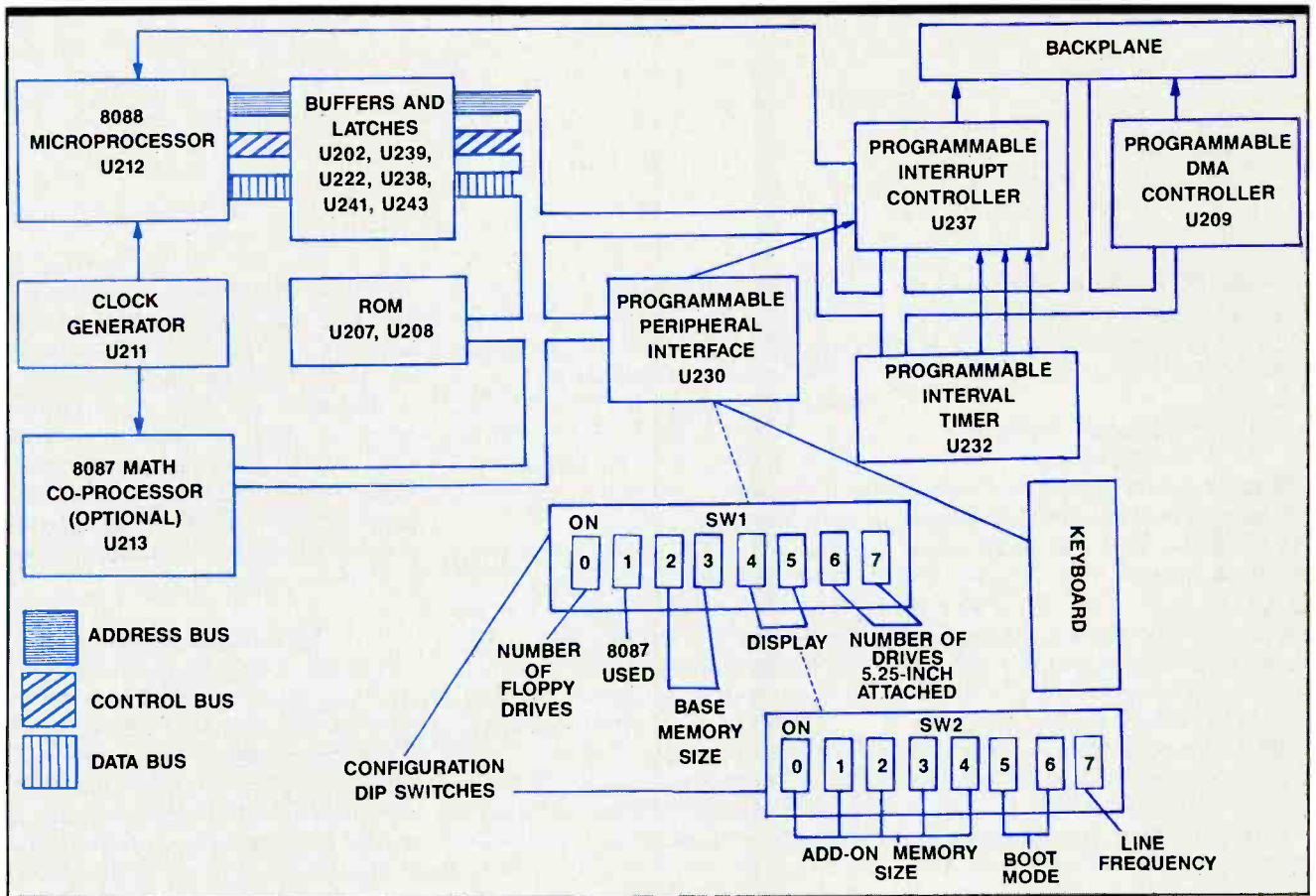
Figure 3. This block diagram of the signal flow in a typical CPU card gives an idea of the communication back and forth through the buses.
