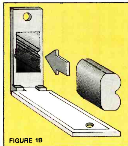
Figure 1. To install a battery in the IBM PC/XT, the servicer must first turn off the system and all external options, then remove the screw that closes the battery compartment (Figure 1A). The battery slides in as shown in Figure 1B, with the terminal end first.
